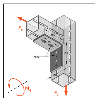
MODFRAME® 4-hole angle from MOD 100
