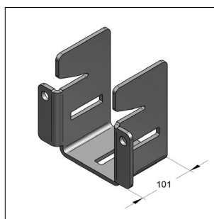
MODFRAME® Clamping shoe single
